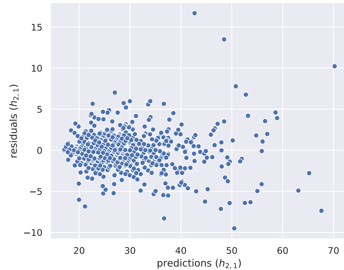
Residual Plot (w/ eng. feat. + PCA)
