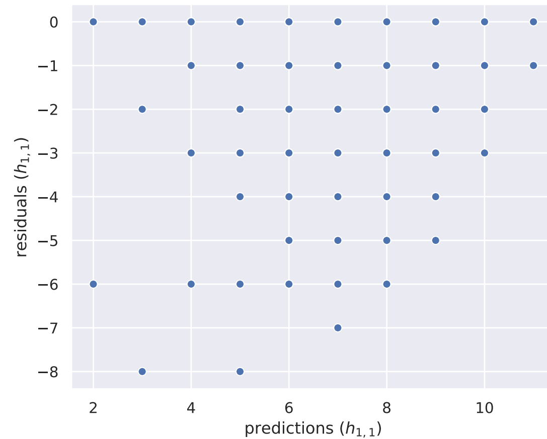
Residual Plot (w/ eng. feat.)
