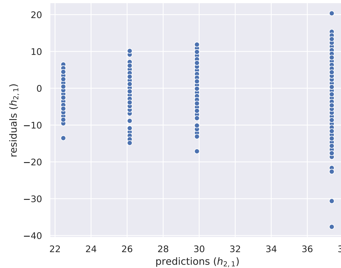
Residual Plot (w/ eng. feat.)
