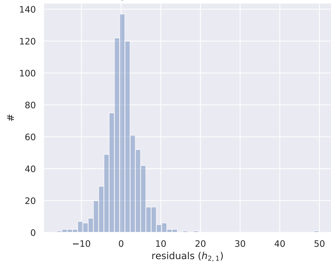
Histogram of the Residuals (w/ proj. spaces)
