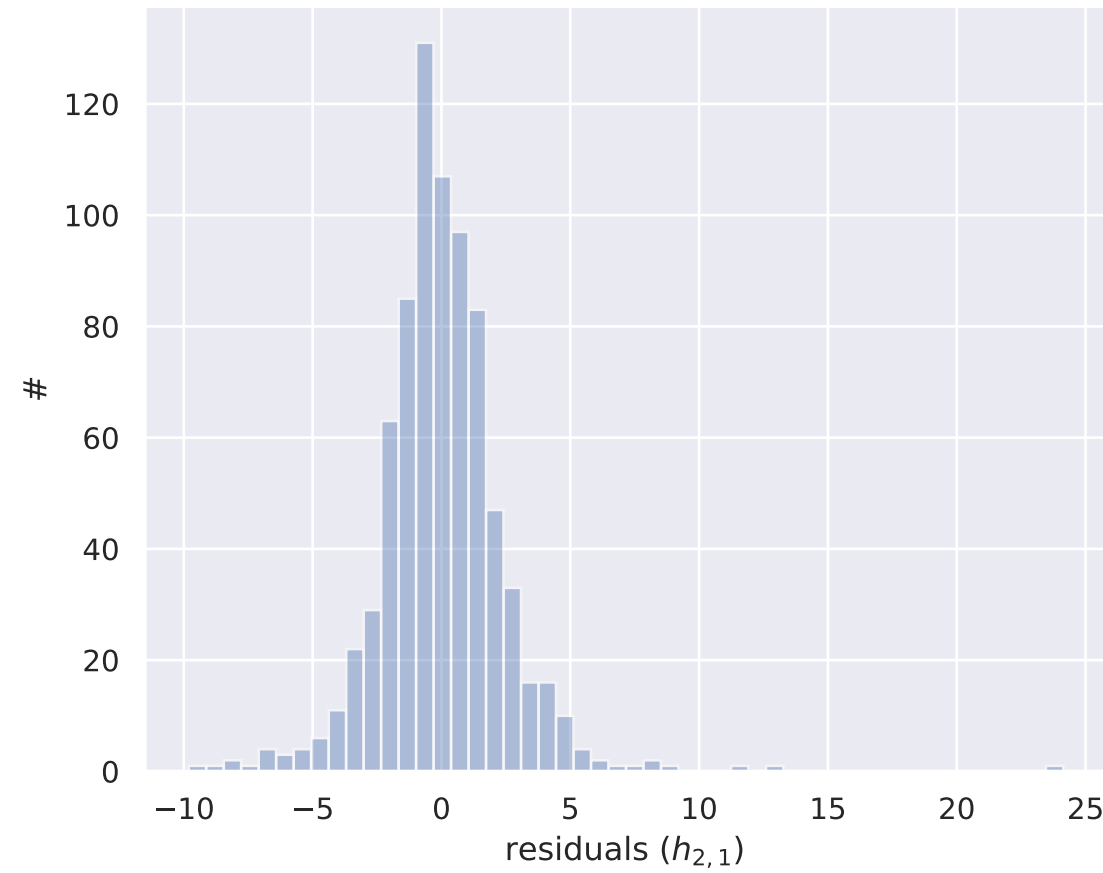
Histogram of the Residuals (w/ eng. feat. + PCA)
