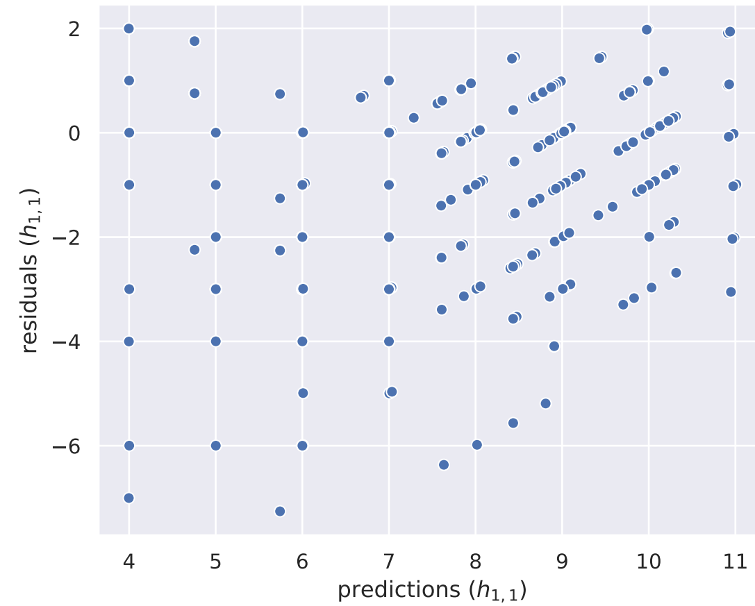
Residual Plot (w/ eng. feat. + PCA)
