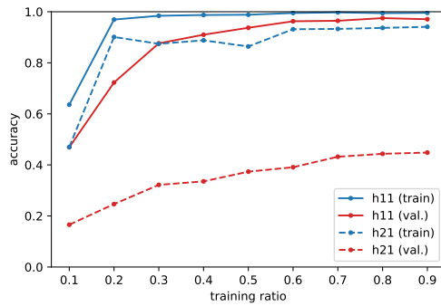
(a) predicting both h^{1,1} and h^{2,1}
