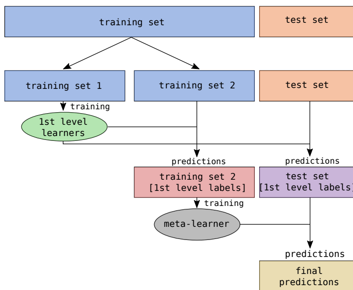
Figure 9.26: Stacking ensemble learning with two level learning.
