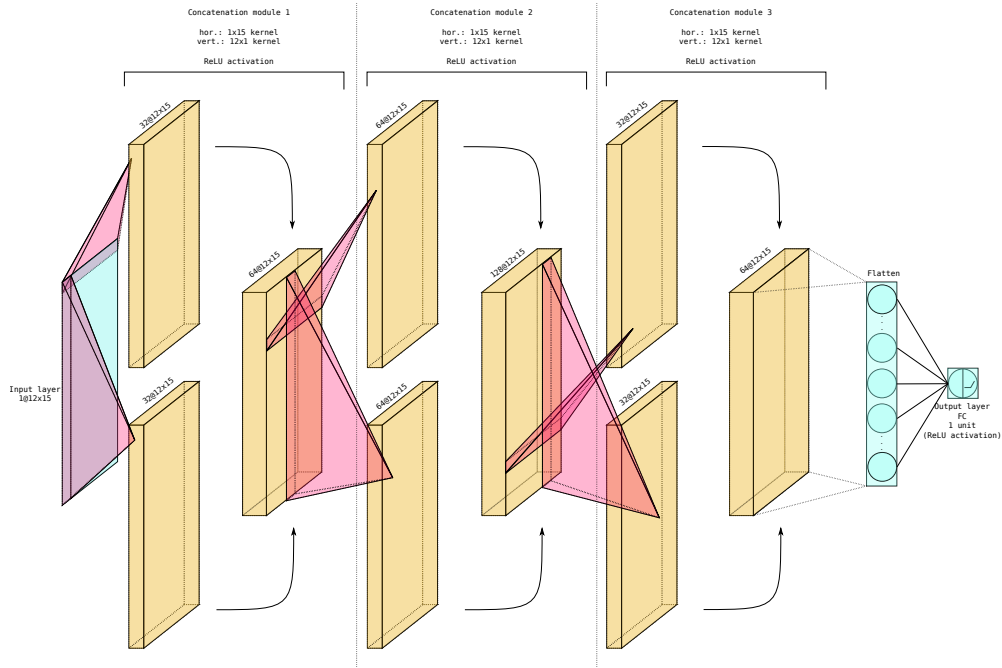
Figure 9.22: In each concatenation module (here shown for the “old” dataset) we operate with separate convolution operations over rows and columns, then concatenate the results. The overall architecture is composed of 3 “inception” modules made by two separate convolutions, a concatenation layer and a batch normalisation layer (strictly in this order), followed by a dropout layer, a flatten layer and the output layer with ReLU activation (in this order).
