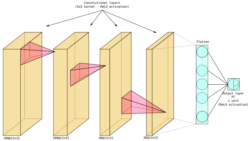
Figure 9.19: Pure convolutional neural network for predicting h^{1,1} . It is made of 4 modules composed by convolutional layer, ReLU activation, batch normalisation (in this order), followed by a dropout layer, a flatten layer and the output layer (in this order).
