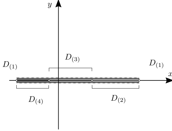
Figure 2.2: Branch cut structure of the complex plane with N_B = 4 . Cuts are pictured as solid coloured blocks running from one intersection point to another at finite.
