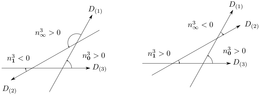
Figure 2.5: The Abelian limit when the triangle has one obtuse angle. This corresponds to the cases n_0 + n_\infty > \frac{1}{2} and n_0 > n_\infty which are exchanged under the parity P_2 .
