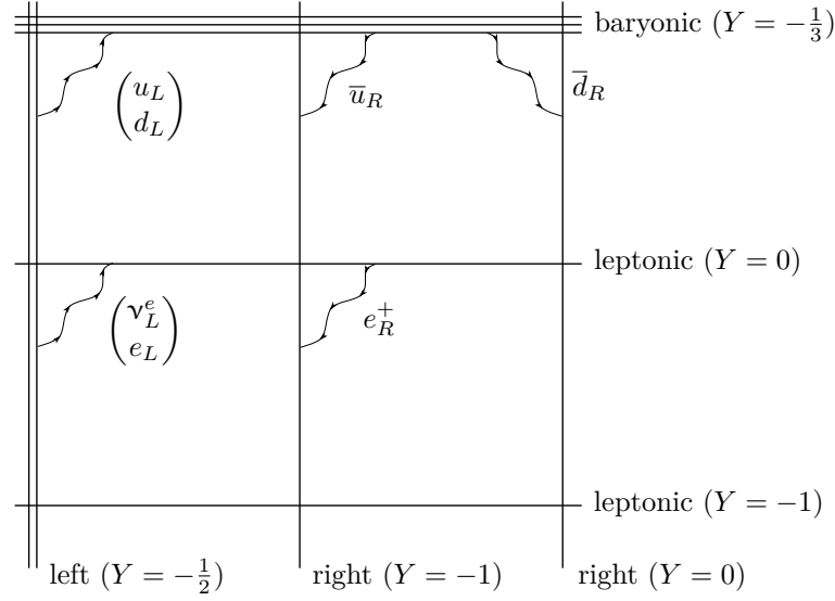
Figure 1.3: Example of SM-like construction using intersecting D-branes with the indications of the hypercharge Y . Perpendicular angles are only a matter of convenience: they are in principal arbitrary.
