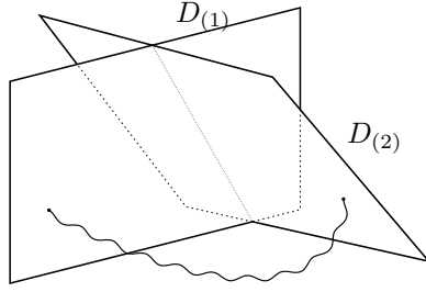
Figure 2.7: Pictorial 3-dimensional representation of two D2-branes intersecting in the Euclidean space \mathbb{R}^3 along a line (in \mathbb{R}^4 the intersection is a point since the co-dimension of each D-brane is 2): since it is no longer constrained on a bi-dimensional plane, the string must be deformed in order to stretch between two consecutive D-branes. Its action can be larger than the planar area.
