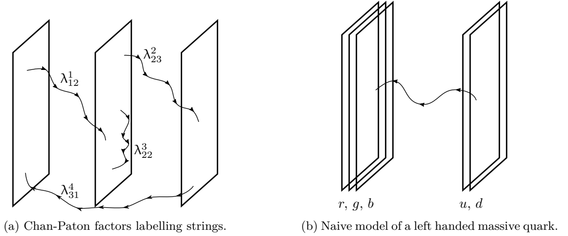
Figure 1.2: Strings attached to different D-branes.
