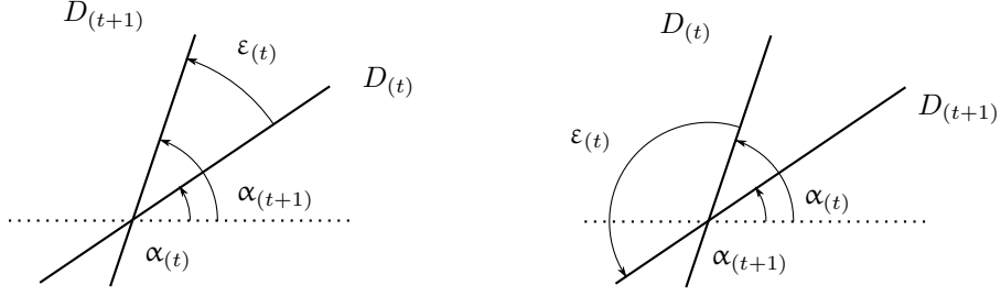
Figure 2.6: The geometrical angles used in the usual geometrical approach to the Abelian configuration do not distinguish among the possible branes orientations. In fact we have 0 \leq \alpha < 1 and 0 < \epsilon < 1 .
