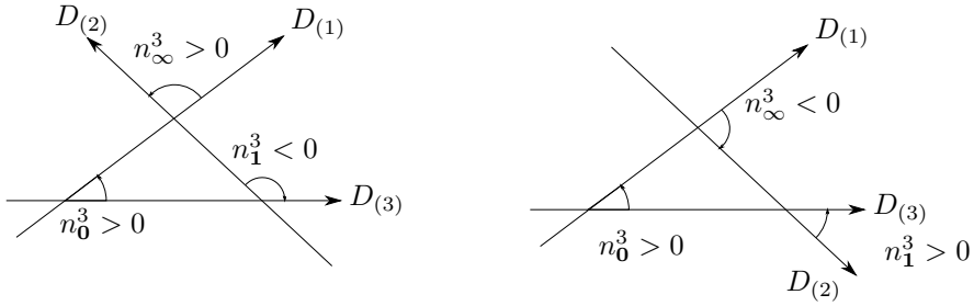
Figure 2.4: The Abelian limit when the triangle has all acute angles. This corresponds to the cases n_0 + n_\infty < \frac{1}{2} and n_0 < n_\infty which are exchanged under the parity P_2 .
