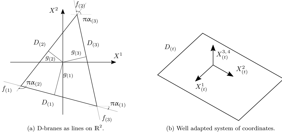
Figure 2.1: Geometry of D-branes at angles.
