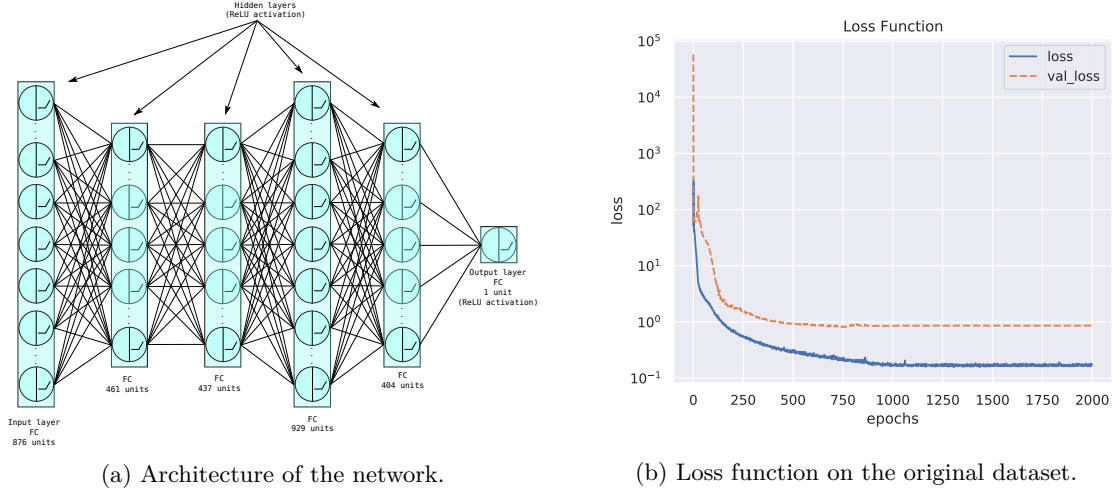
Figure 9.18: Fully connected network for the prediction of h^{1,1} . For simplicity we do not draw the dropout and batch normalisation layers present after every densely connected layer.
