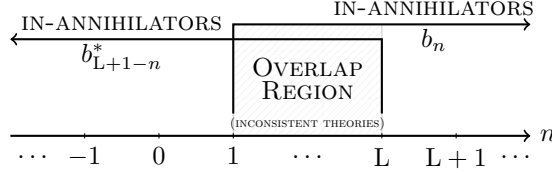
Figure 3.3: As a consistency condition, we have to exclude the values of L for which both b_n^{(E)} and b_{L+1-n}^{*(\bar{E})} are in-annihilators with a non vanishing anti-commutation relation.
