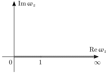
Figure 2.3: Fixing the \text{SL}_2(\mathbb{R}) invariance for N_B = 3 and \bar{t} = 1 leads to a cut structure with all the cuts defined on the real axis towards \omega_{\bar{t}} = \infty .
