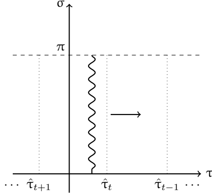
Figure 3.1: Propagation of the string in the presence of the worldsheet defects.
